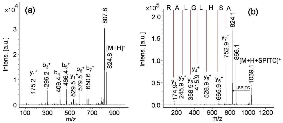
Figure S5: ASHLGLAR model peptide fragmentation (a) without and (b) with SPITC derivatization
