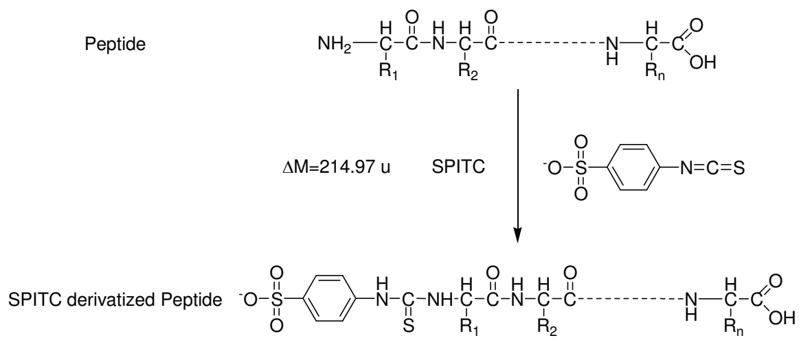
Figure S1: SPITC derivatization of peptides
