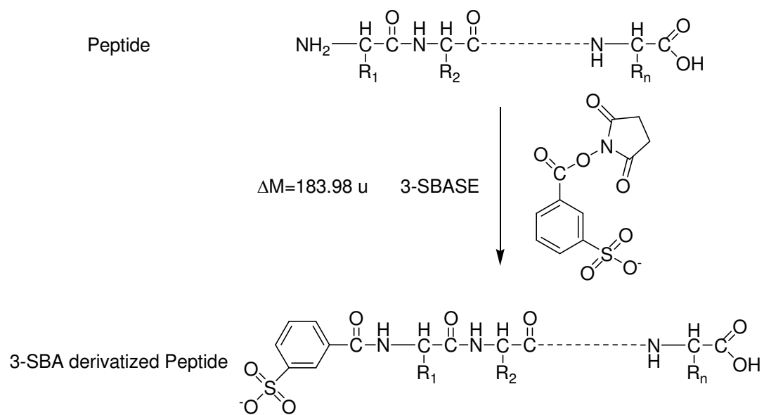
Figure S2: 3-SBA derivatization of peptides
