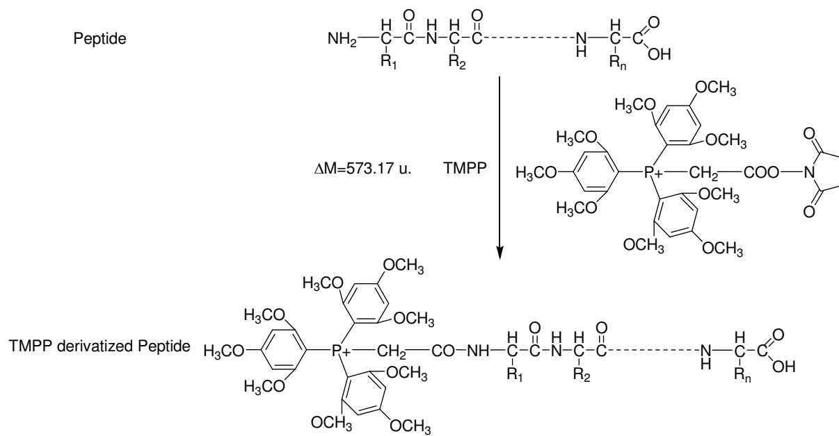
Figure S3: TMPP derivatization of peptides
